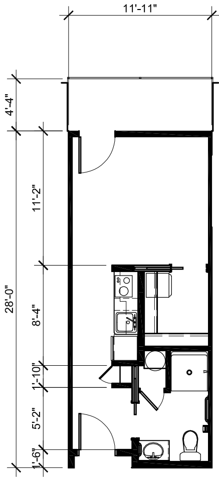
STUDIO - UNIT A 3 UNITS IN BUILDING 330 SQ FT 45 SQ FT DECK
